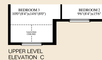
OPT. UPPER LEVEL W/3 BATHROOMS ELEVATION C
