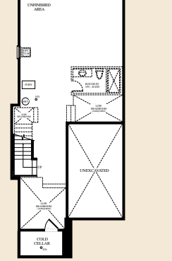
LOWER LEVEL ELEVATION A, B & C
