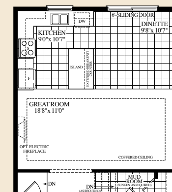
MAIN LEVEL FOR OPT. KITCHEN LAYOUT
