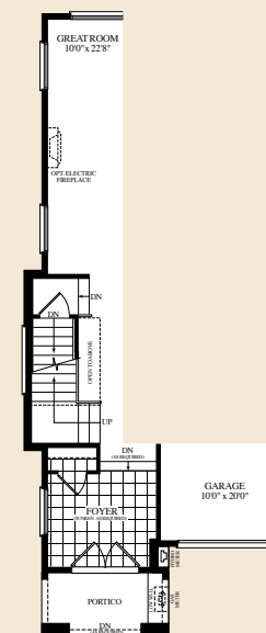
MAIN LEVEL ELEVATION C
