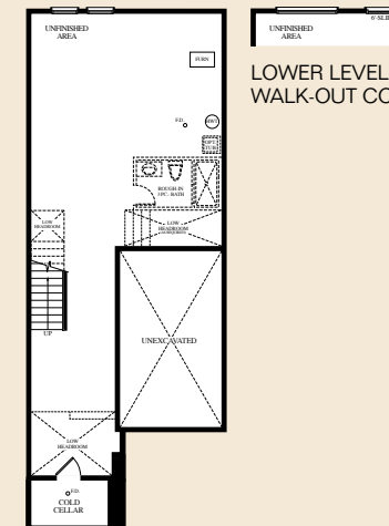
LOWER LEVEL ELEVATION A, B & C
