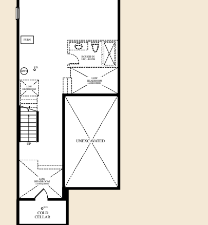
LOWER LEVEL ELEVATION A, B & C
