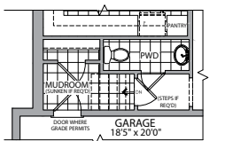
PARTIAL MAIN FLOOR MUDROOM W/ADDITIONAL RISERS
