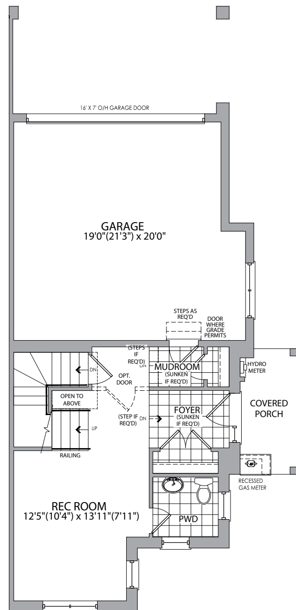
LOWER FLOOR ELEV. A
